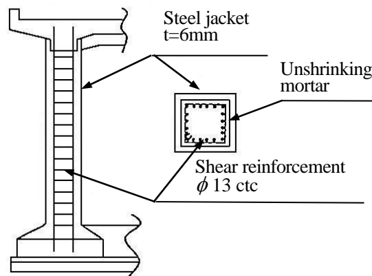
Figure 1. Column retrofitted with steel jacket
